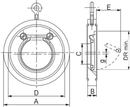
Connection flange
